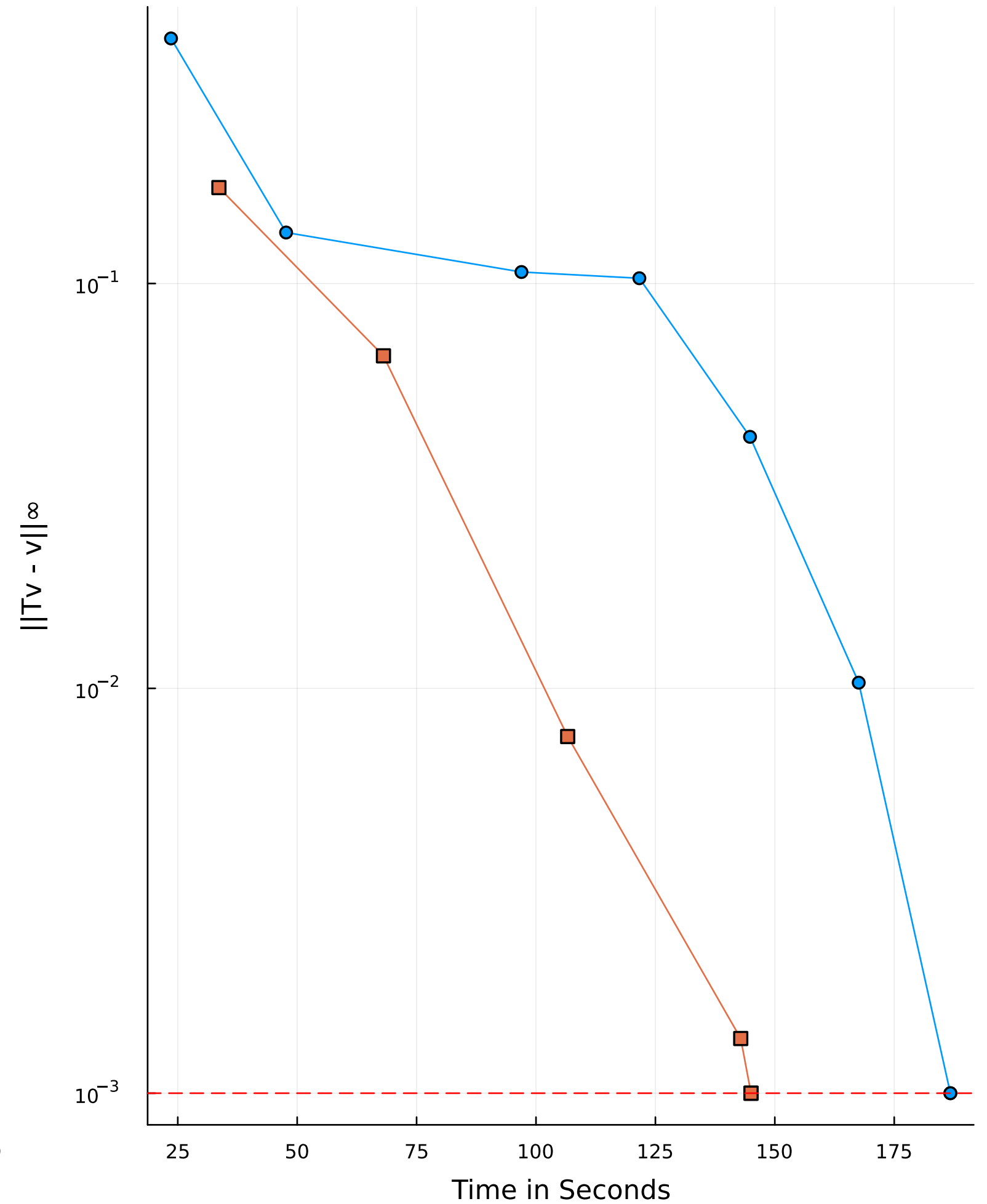
Large Problems
