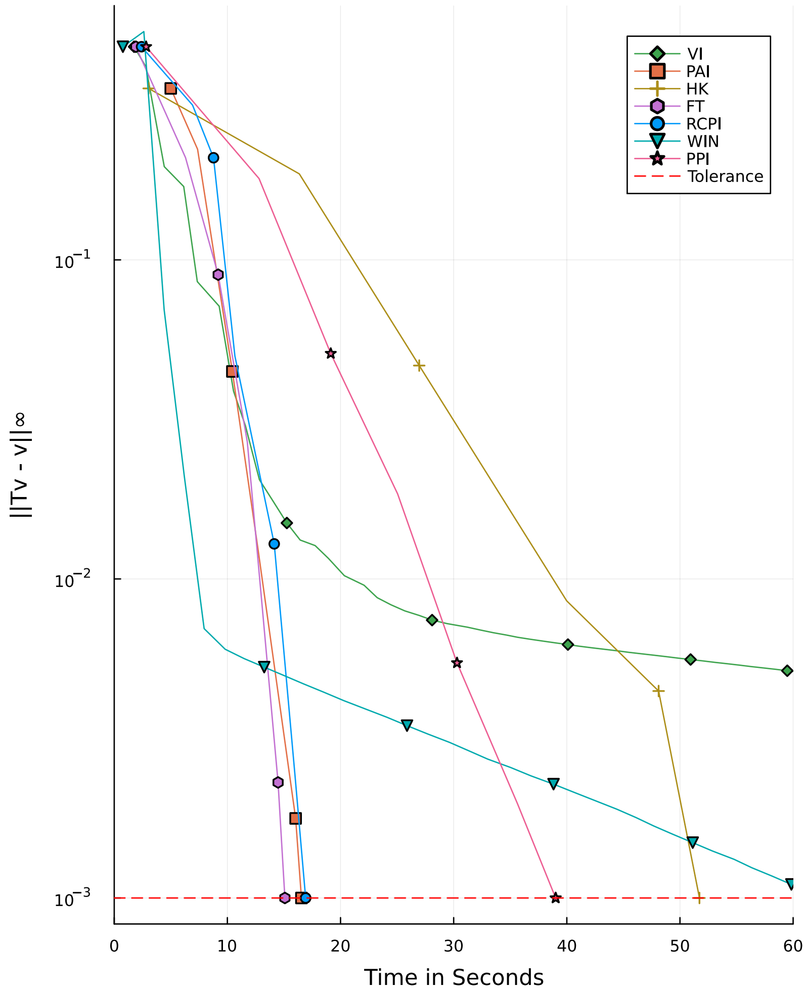
Small Problems
